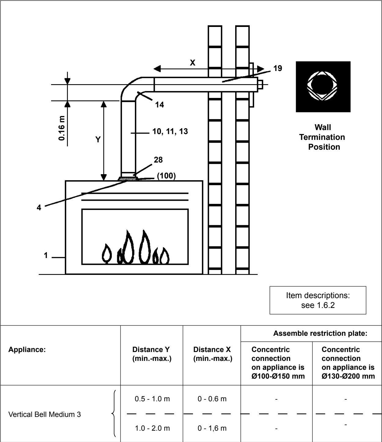
Figure 10: Horizontal wall termination
