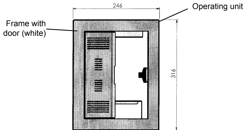
Figure 15: Operating unit
