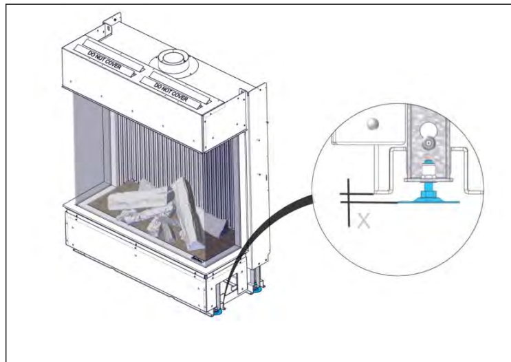
Figure 23. Aligning with adjustable feet
