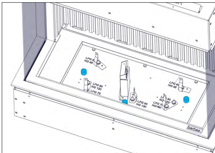
Figure 41. Position of ambient light bulbs
